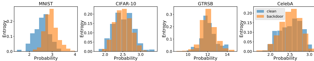
Figure 12: STRIP against all-to-all scenario.
