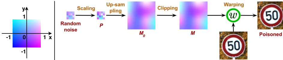
Figure 2: Process of creating the warping field M and using it to generate poisoned images.
