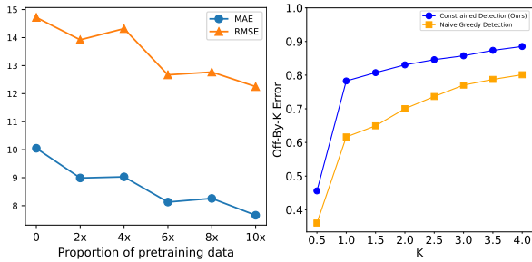
Figure 4: Left: model’s performance as the amount of pretraining data is increased; “2x” represents twice the size of the real training set. Right: Quantitative result on temporal location detection. Off-By-K error under varying K.
