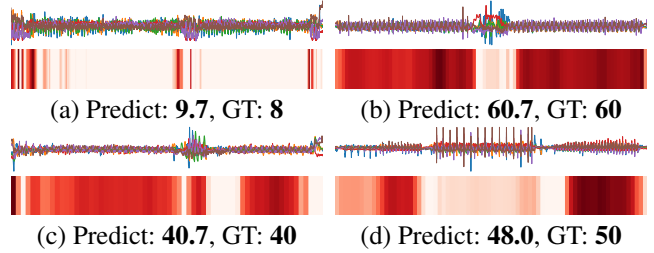
Figure 5: Qualitative results. Four prediction examples. Each example shows the input sensor data, the estimated density map, the predicted count, and the ground truth value.
